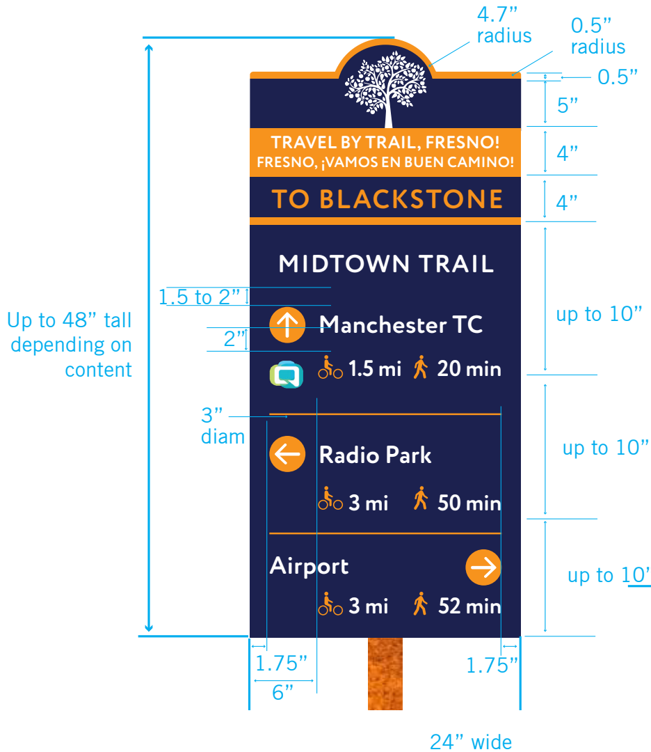
Figure 37: Trail Welcome Sign Layout
