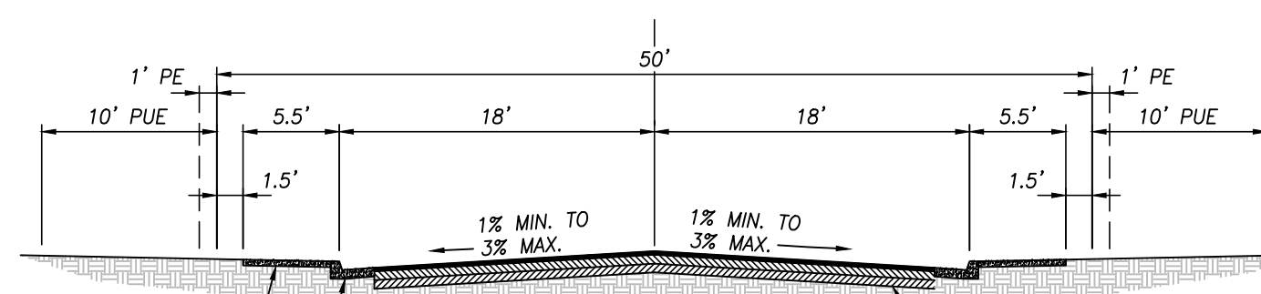
TYPICAL LOCAL STREET
