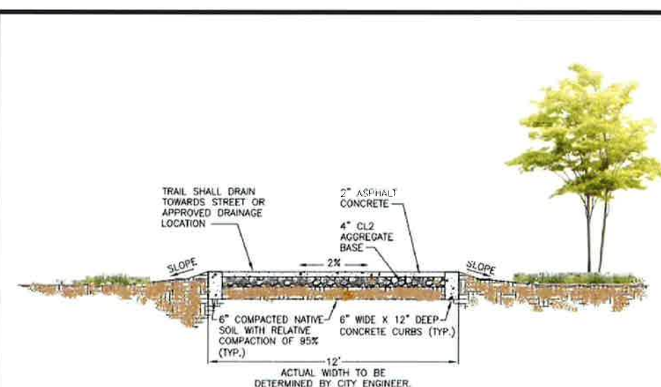
ASPHALT MULTIPURPOSE TRAIL
