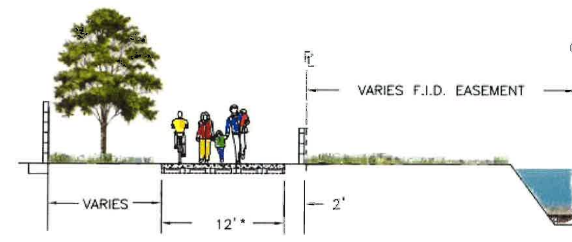
TRAIL CROSS SECTION ADJACENT TO CANAL
