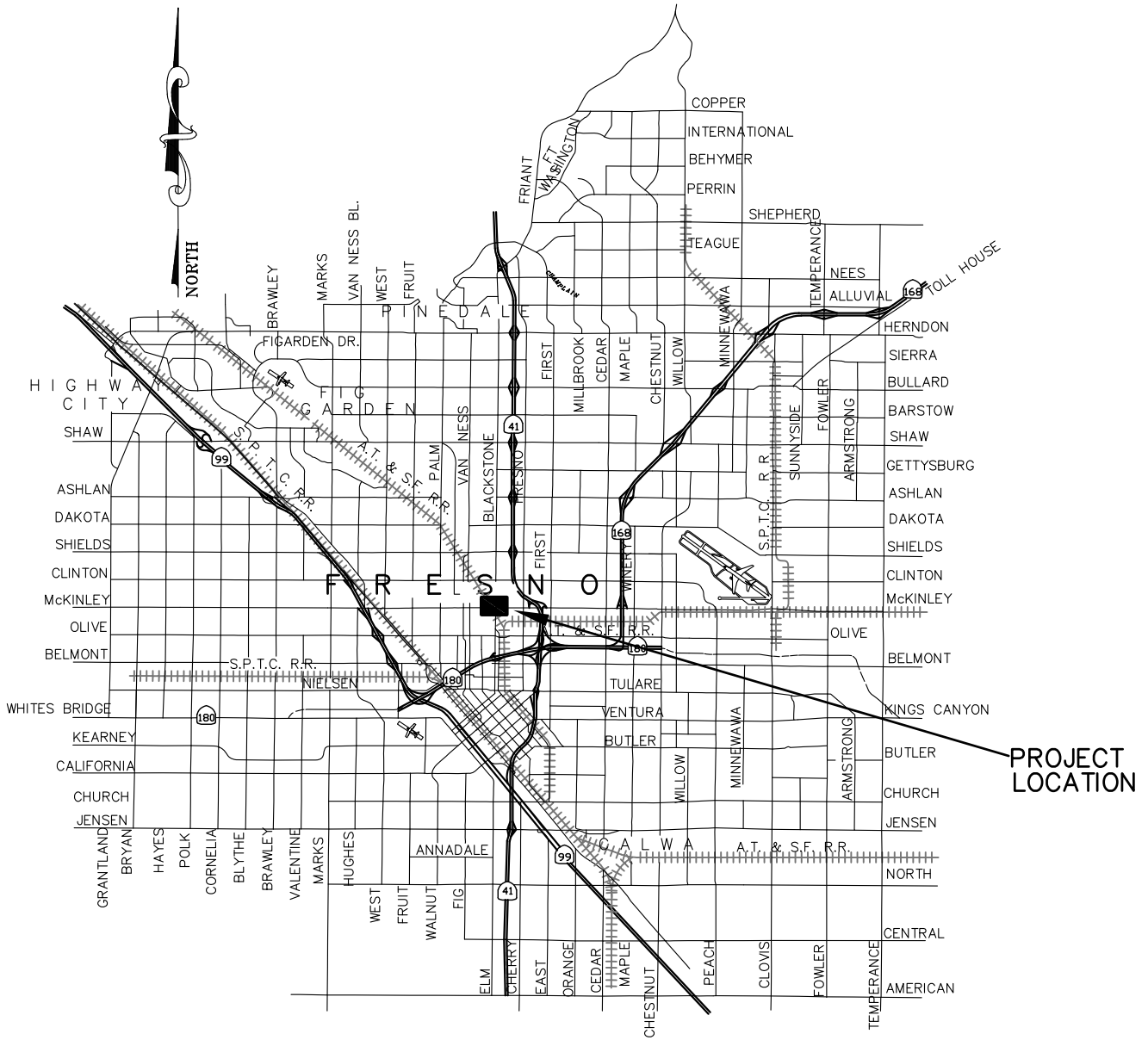
VICINITY MAP
