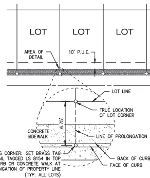
WITNESS CORNER DETAIL FOR FRONT YARDS
