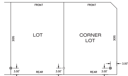
WITNESS CORNER DETAIL FOR DURABLE MONUMENT
