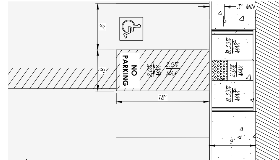
A TYPICAL VAN ACCESSIBLE PARKING STALL NOT TO SCALE NOTE: THE FIRST REQUIRED ACCESSIBLE PARKING SPACE SHALL BE VAN ACCESSIBLE
