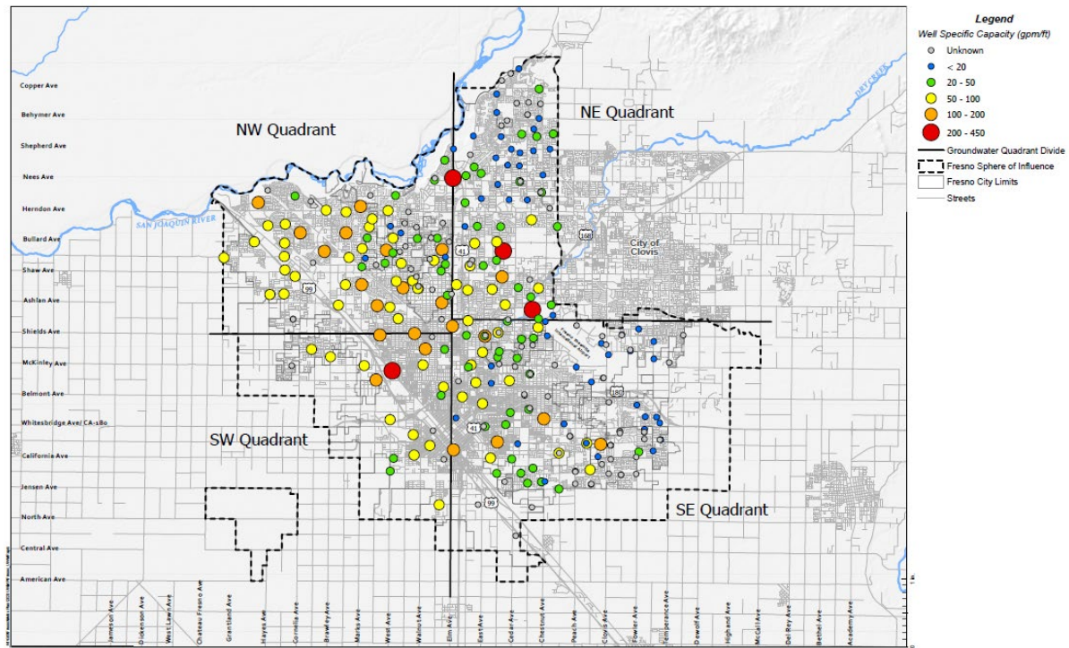
Figure 4: City Wells Specific Capacity
