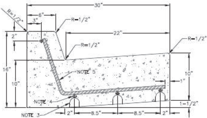
REINFORCED CURB AND GUTTER DETAIL
