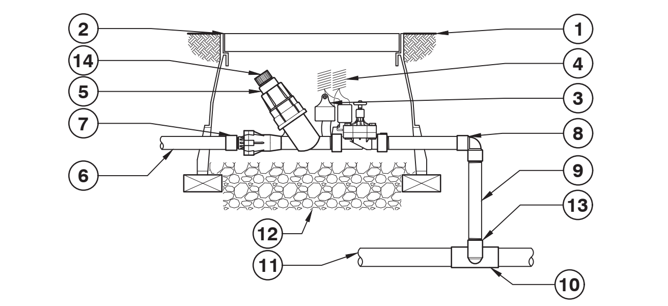
5 17MM EZ-ID DRIPLINE AIR RELIEF VALVE NOT TO SCALE P-CO-CIR-02
