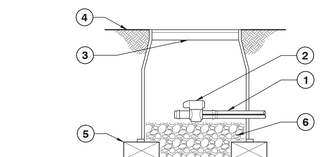
3 FLOW SENSOR 3/4" = 1'-0" P-CO-CIR-03
