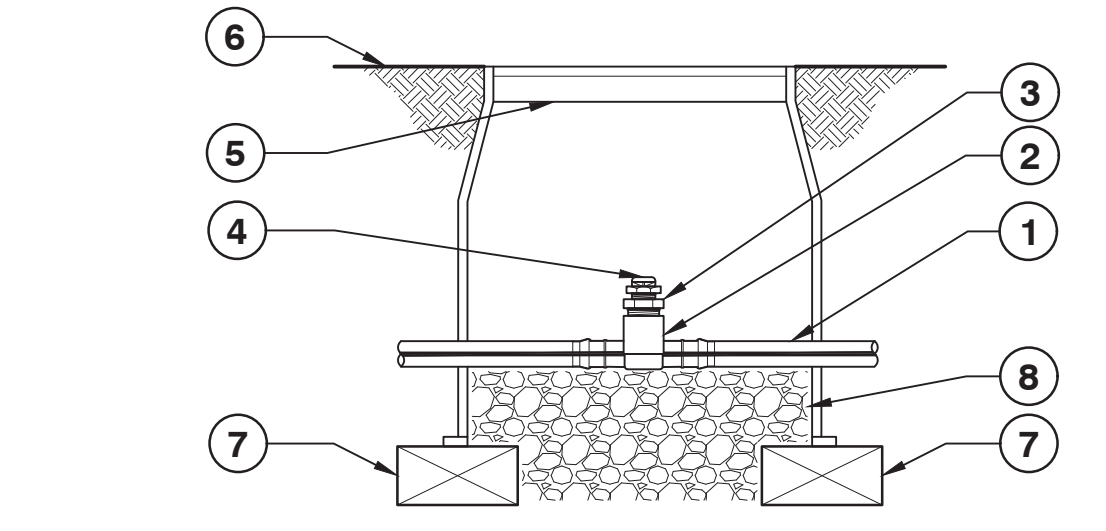
2 MASTER CONTROL VALVE AND FLOW SENSOR ASSEMBLY 1" = 1'-0" P-CO-CIR-01
