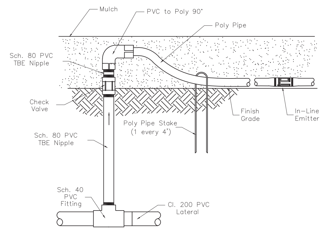
8 PVC TO POLY CONNECTION 3" = 1'-0" P-CO-CIR-11
