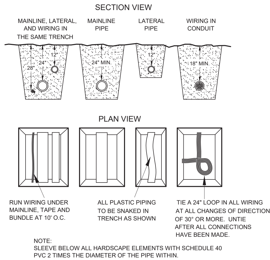
3 PIPE AND WIRE TRENCHING NTS P-CO-CIR-10
