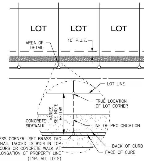
WITNESS CORNER DETAIL FOR FRONT LOT
