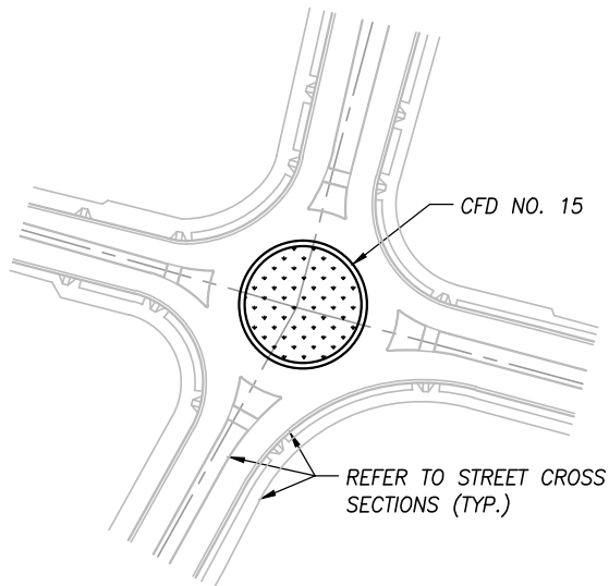
TYPICAL ROUNDABOUT - PLAN VIEW NOTE: ROUNDABOUT SHOWN FOR REFERENCE ONLY.
