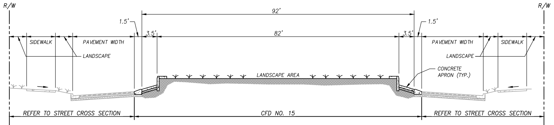
⑧ TYPICAL ROUNDABOUT (CROSS SECTION REFERS TO APPROXIMATE ROUNDABOUT SIZE) ALICANTE AND CLUB HOUSE DRIVE ALICANTE AND ROAD 'G' ROAD 'G' TO WILLOW AVENUE
