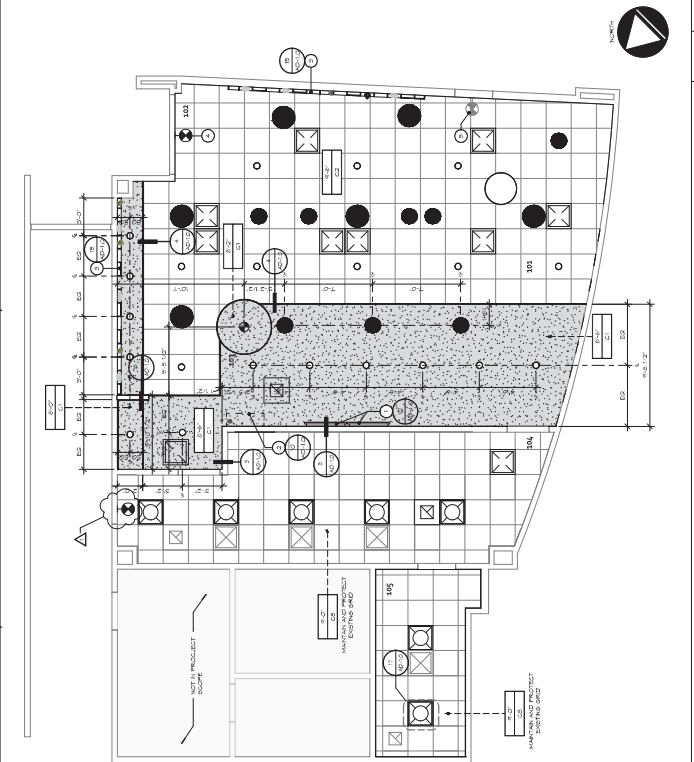
Proposed RCP 1/8" = 1'-0"
