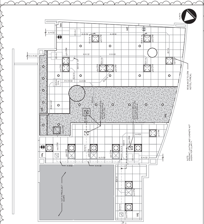
Mechanical Plan 1/8" = 1'-0"
