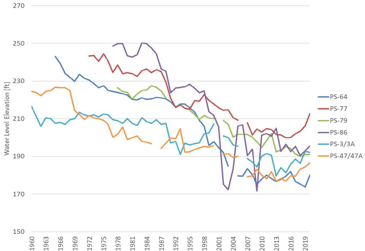
Figure 5: Time Series of Groundwater Levels at Representative Wells
