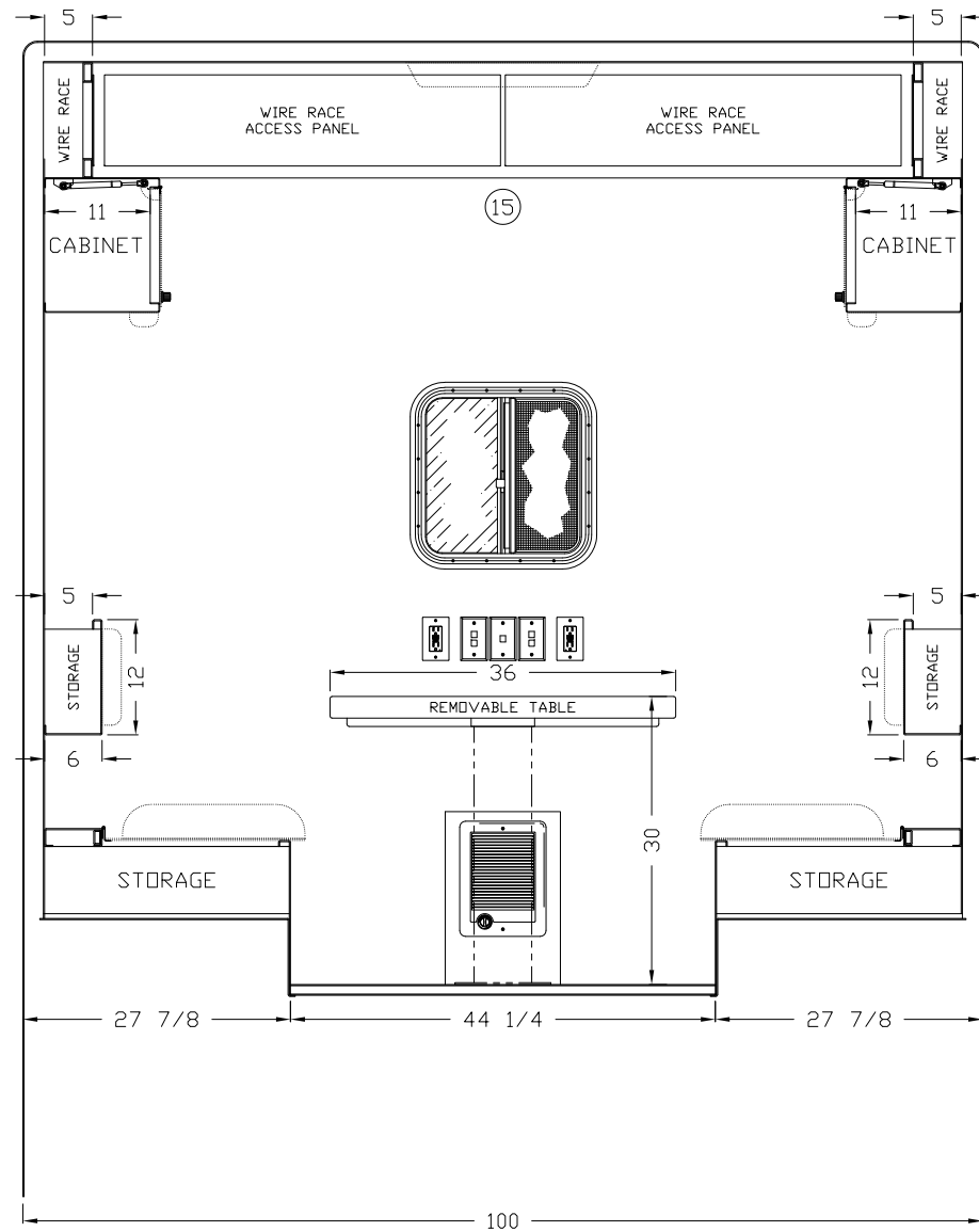
SECTION A - A AFT REAR VIEW
