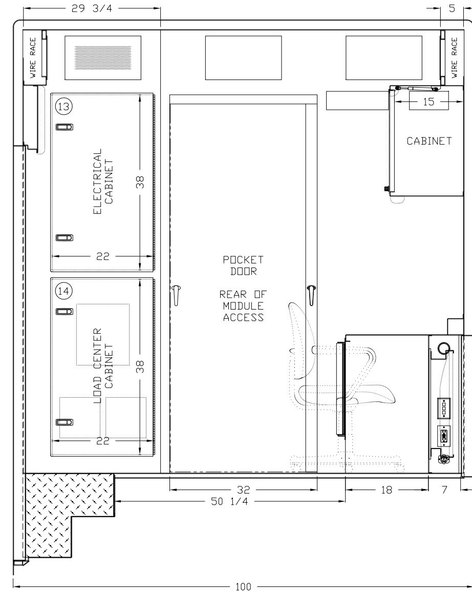
SECTION B - B MIDDLE REAR VIEW
