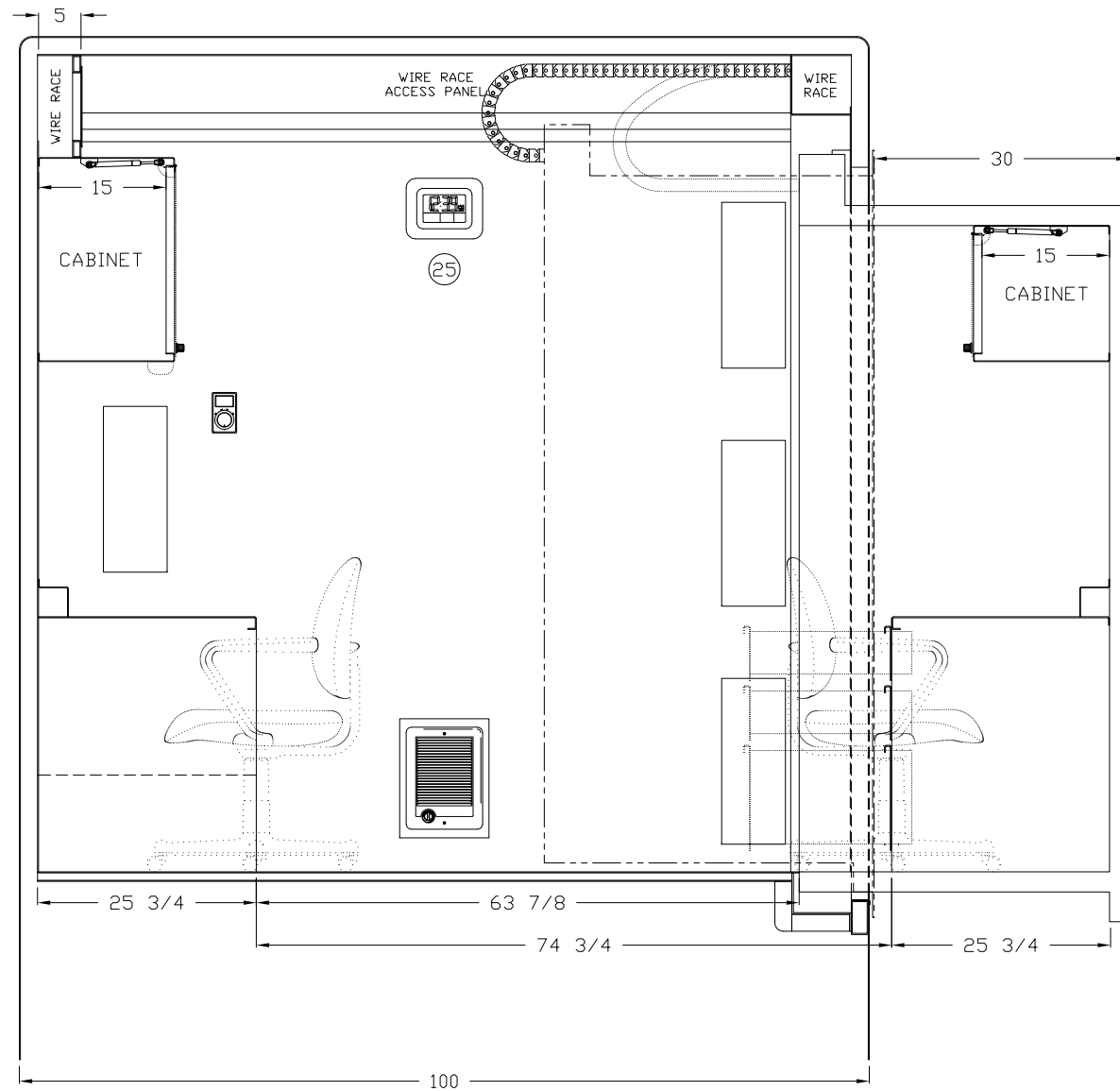
SECTION D - D FORWARD FRONT VIEW
