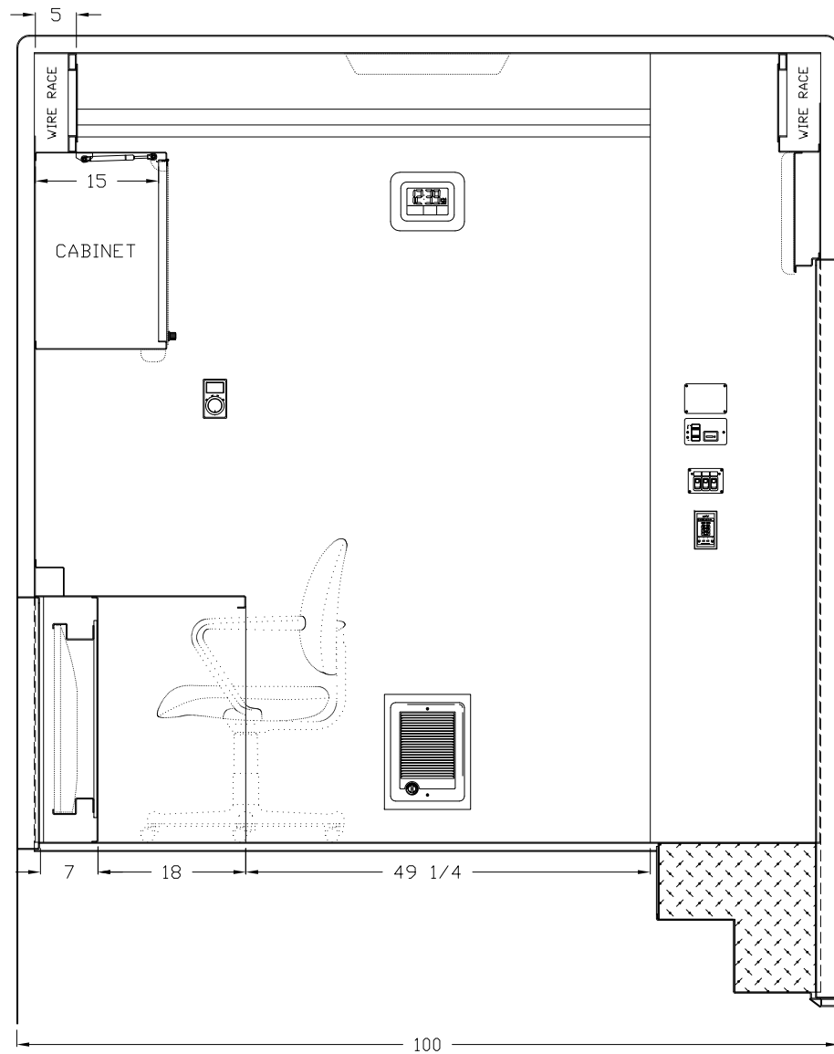
SECTION C - C MIDDLE FRONT VIEW
