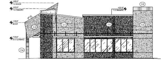
3 WEST ELEVATION AT PLAZA
