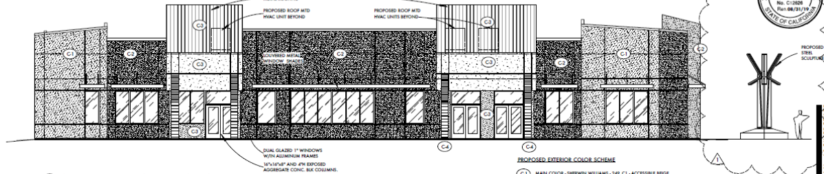
2 NORTH ELEVATION - AT CLINTON
