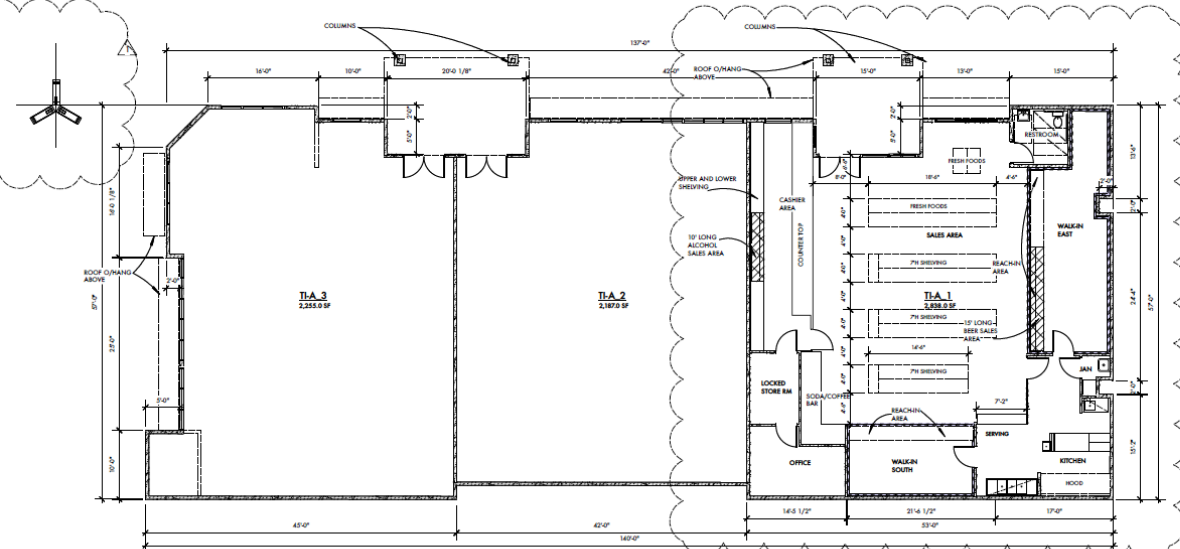
5 BUILDING 'A' SHELL FLOOR PLAN - 7,753.00 SF
