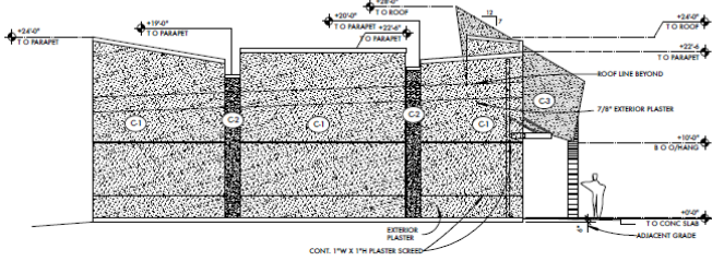
1 EAST ELEVATION AT BLYTHE
