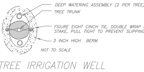
TREE IRRIGATION WELL
